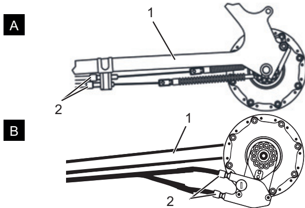
Figure 74: Adjusting sleeves (2) on two alternative versions (A and B) of a dual-cable cable-operated gear shift on the chain stay (1)
