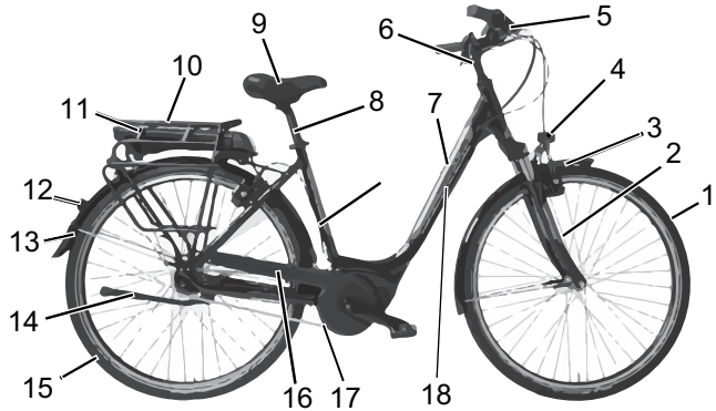
Figure 2: Bicycle, viewed from the right, example of City Cruiser
