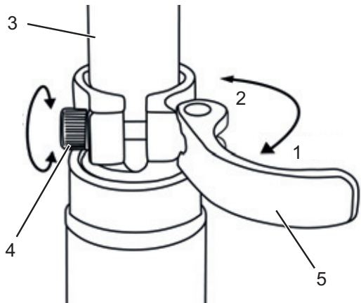
Figure 38: Seat post quick release (3) with clamping lever (5) and adjustment screw (4) in the open position (1) and in the direction of the closed position (2)
