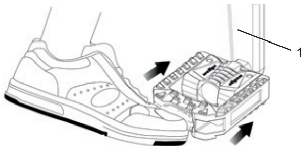
Figure 59: Pushing the pedal against the pedal crank (1)
