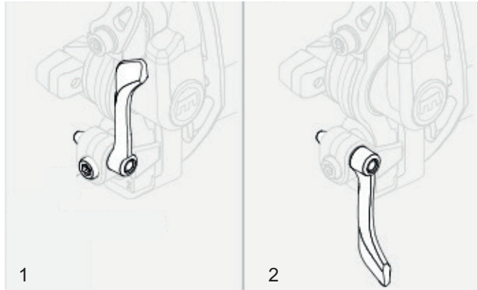
Figure 8: Rim brake locking lever, closed (1) and open (2)
