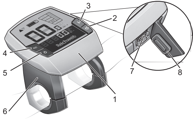
Overview of the structure of the display's operating elements
