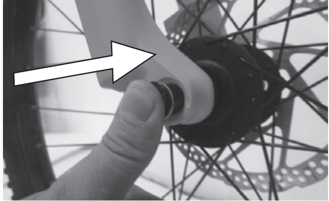
Fully inserting the axle
