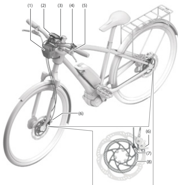
Figura 13: ABS BOSCH
