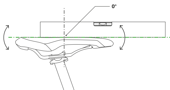
Figure 102: Horizontal saddle tilt with 0° tilt in the centre of the saddle
