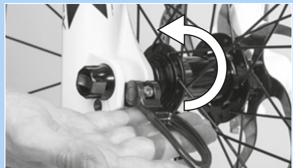
Figure 68: Pressing the quick release lever in the direction of the arrow
