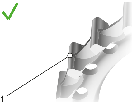
Figure 179: Optimum tooth profile
