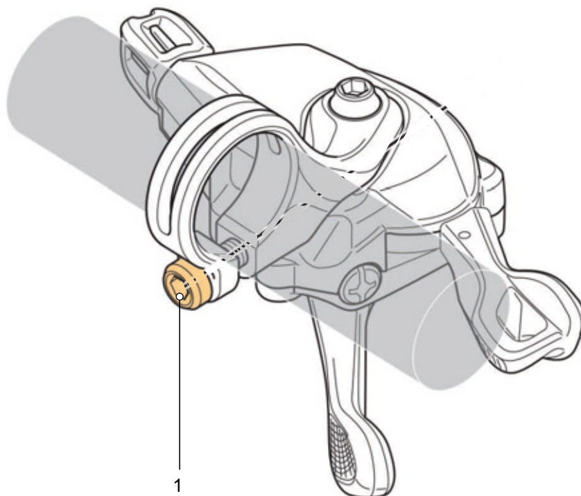
Figure 118: Position of attachment screw in SHIMANO shifter (1)
