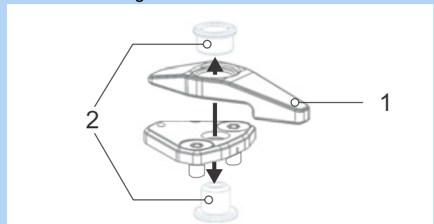
Figure 78: Connect locking lever with base plate
