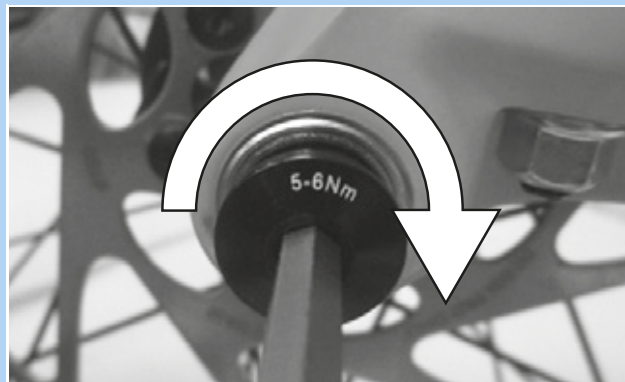
Figure 64: Tightening the securing screw
