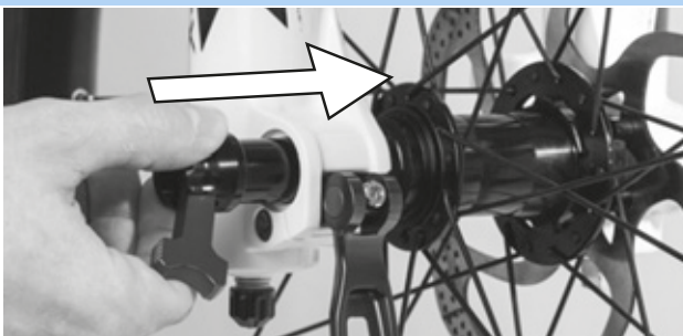
Figure 65: Inserting the cross axle in the direction of the arrow
