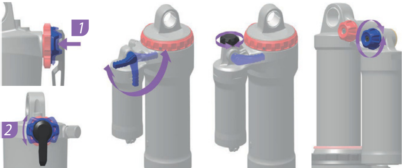
Figure 240: Position and shape of the compression adjuster (blue) depends on the model
