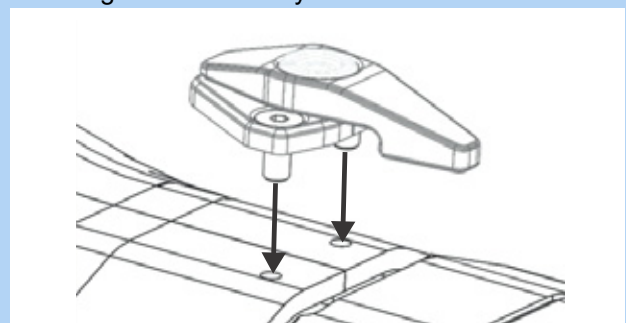
Figure 79: Screwing lever to frame
