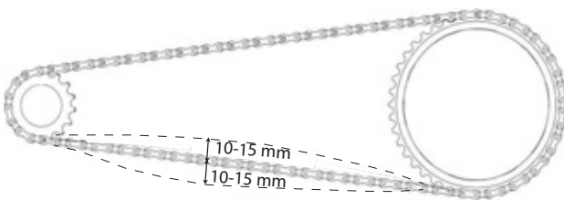
Figure 168: Checking the chain tension (example): 5 mm upwards, 10 mm downwards = 15 mm deviation
