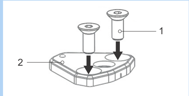
Figure 77: Inserting countersunk screws into base plate
