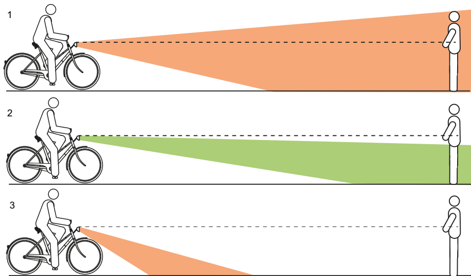
Figure 128: Light positioned too high (1), correctly (2) and too low (3)
