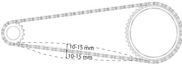
Figure 190: Checking the chain tension
