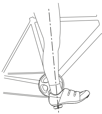
Figure 97: Heel method
