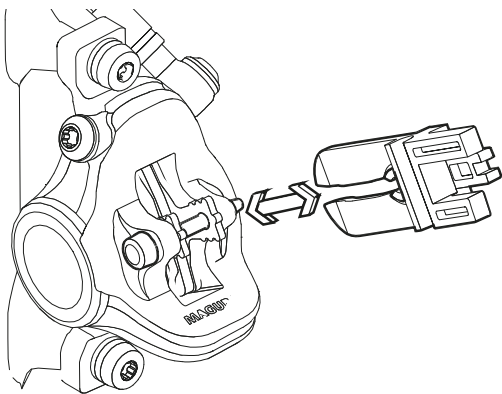
Figure 68: Fastening the transport securing device
