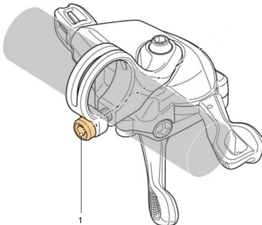
Figure 128: Position of attachment screw in SHIMANO shifter (1)
