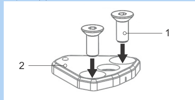
Figure 87: Inserting countersunk screws into base plate
