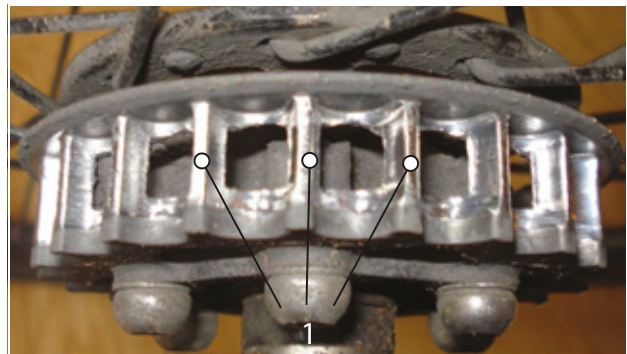
Figure 185: Photo showing example of worn tooth profile
