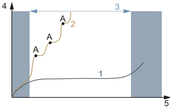
Figure 164: Diagram showing wear, operating hours (x) vs. material abrasion (y)
