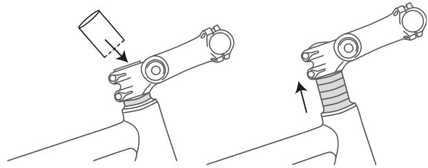
Figure 118: Raising the Ahead stem by fitting spacer rings
