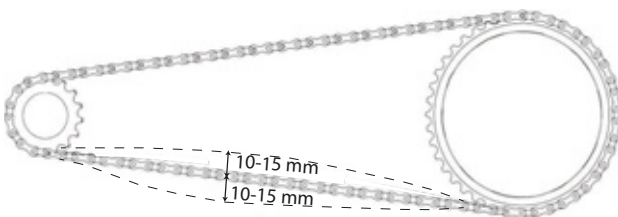
Figure 172: Checking the chain tension (example): 5 mm upwards, 10 mm downwards = 15 mm deviation
