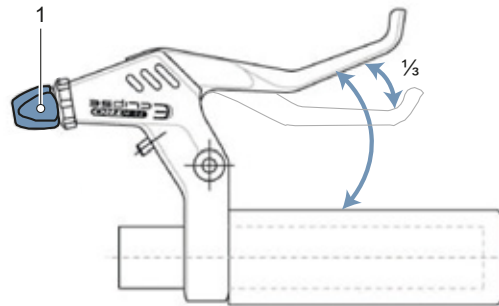
Figure 171: Turn setting screw (1) until brakes initiate after \frac{1}{3} of the handbrake distance is reached
