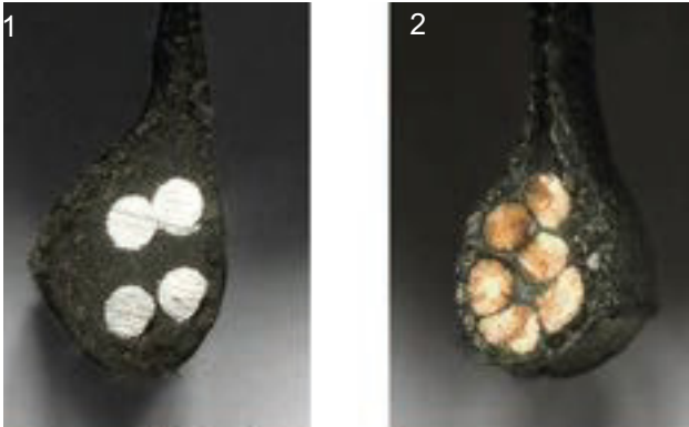
Figure 25: Steel bead core (1) and Kevlar bead core (2)
