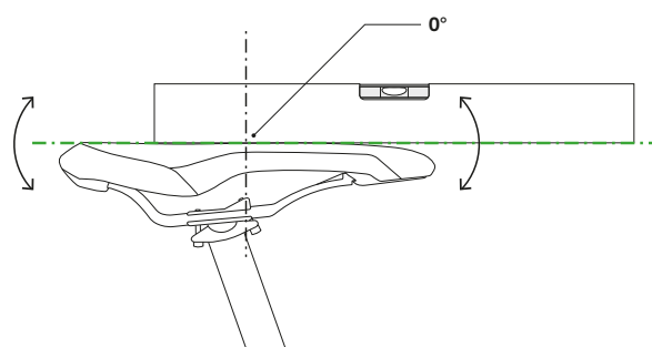
Figure 112: Horizontal saddle tilt with 0° tilt in the centre of the saddle
