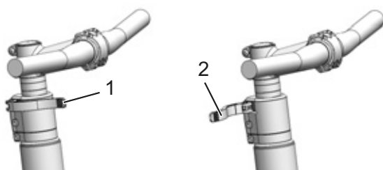
Figure 115: Open (2) and closed (1) stem clamping lever; All Up used as an example
