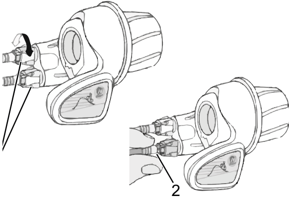
Figure 198: Twist grip with adjusting sleeves (1) and play in the gear shift (2)
