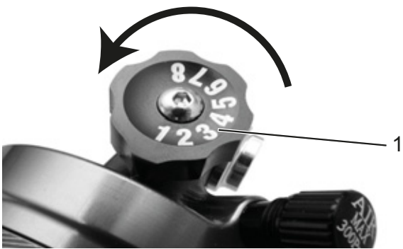
Figure 226: SR SUNTOUR compression adjuster (1) on the rear frame damper
