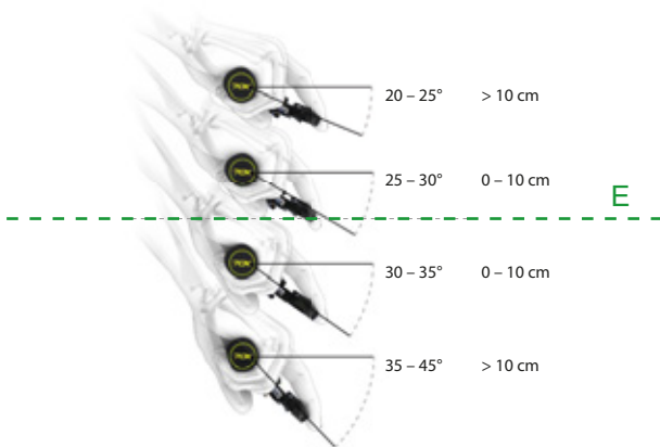
Figure 126: Brake angle
