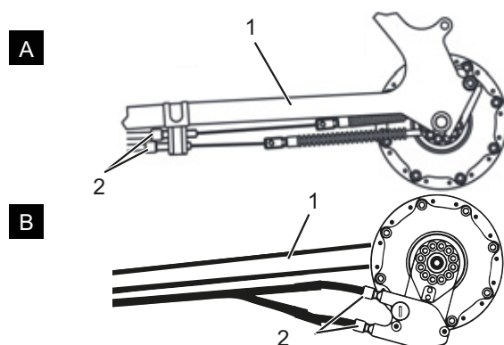
Figure 197: Adjusting sleeves (2) on two alternative versions (A and B) of a dual-cable, Bowden-cable-operated gear shift on the chain stay (1)
