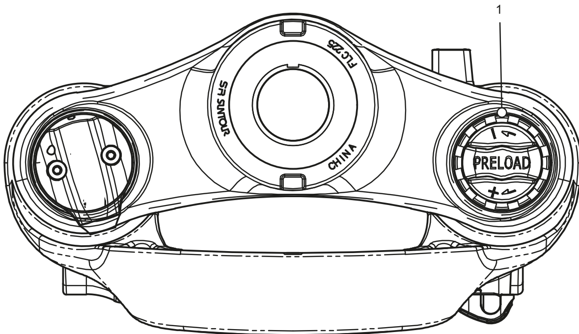
Figure 129: Sag setting wheel (1) on the suspension fork crown
